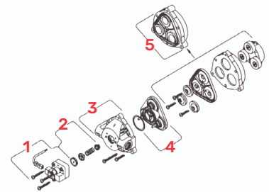
8000 SERIES PUMP
